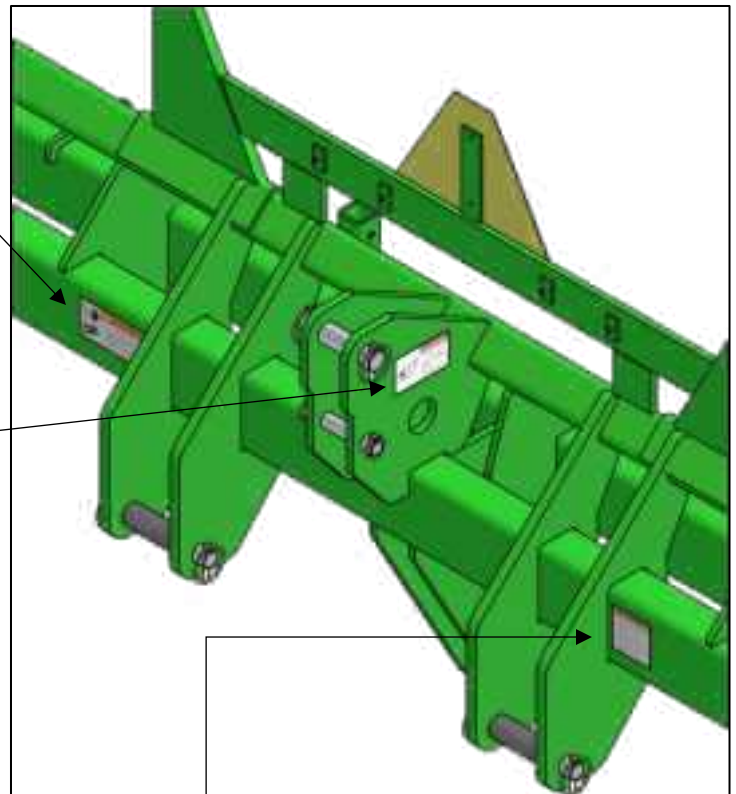
3-Point Hitch
